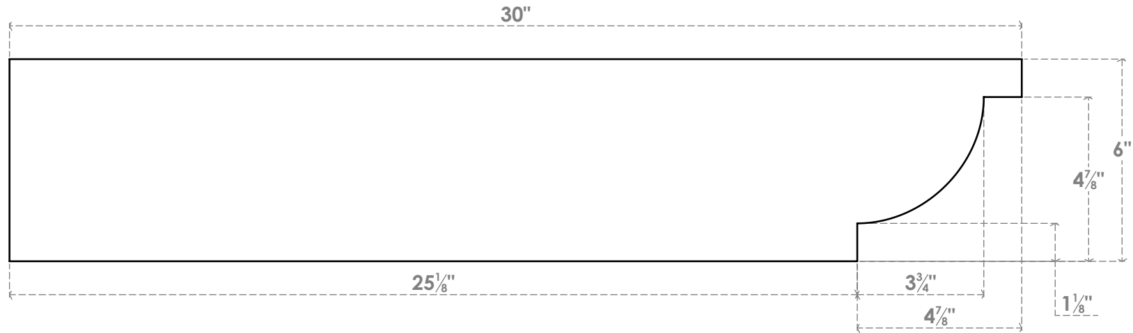
SIDE PROFILE
